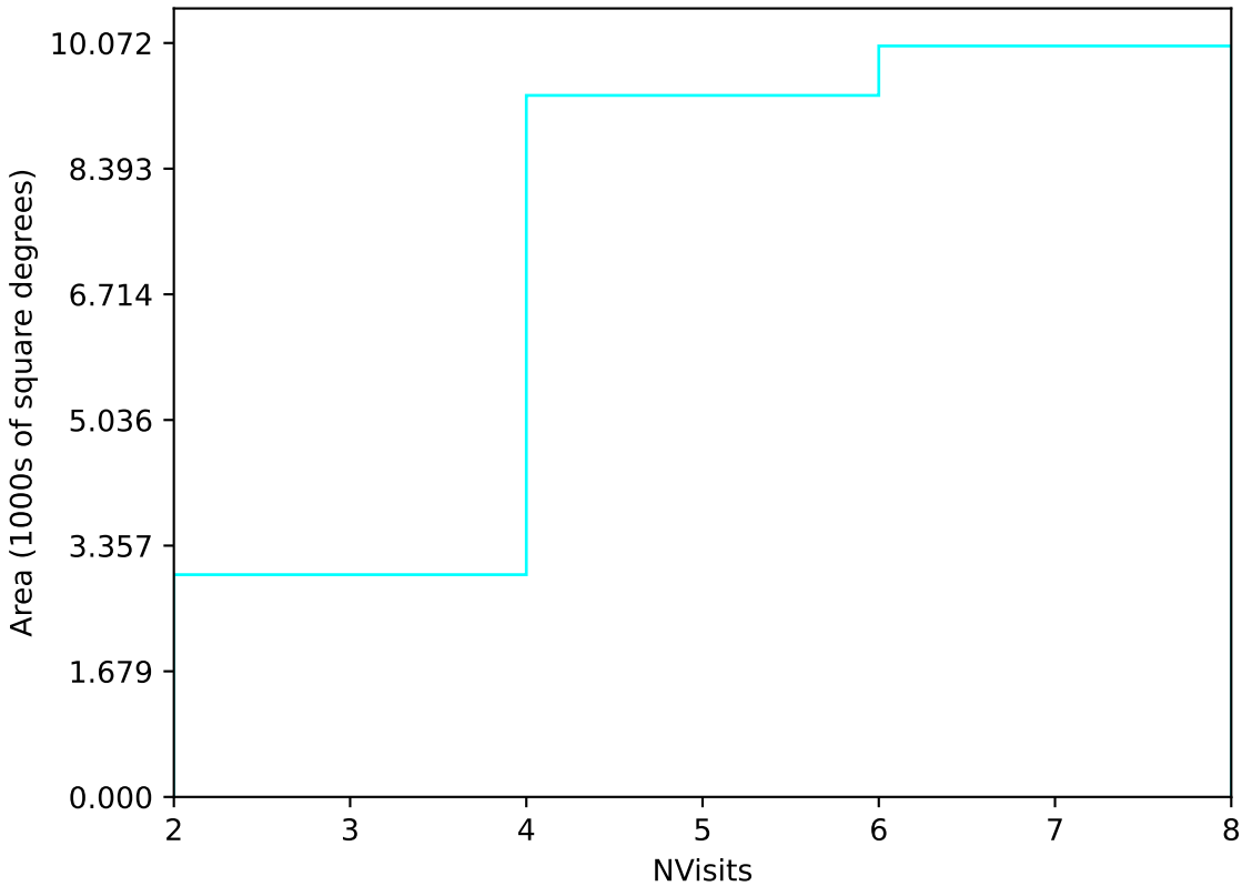
roll_pause_mjdp270_v3.4_10yrs Yr 1 u band: NVisits
