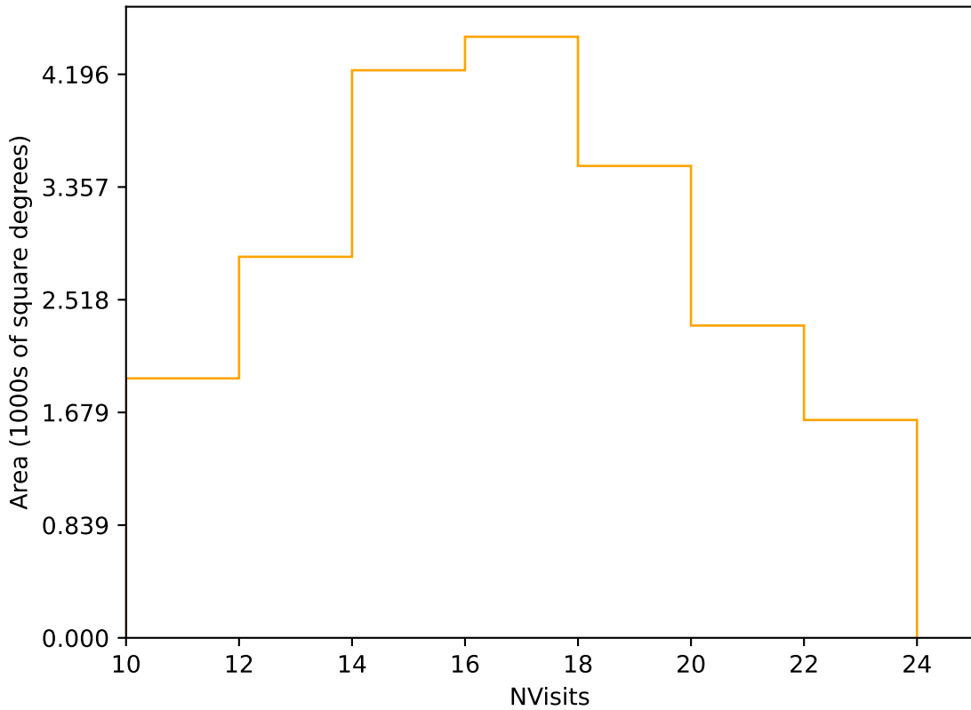
roll_pause_mjdp270_v3.4_10yrs Yr 1 r band: NVisits
