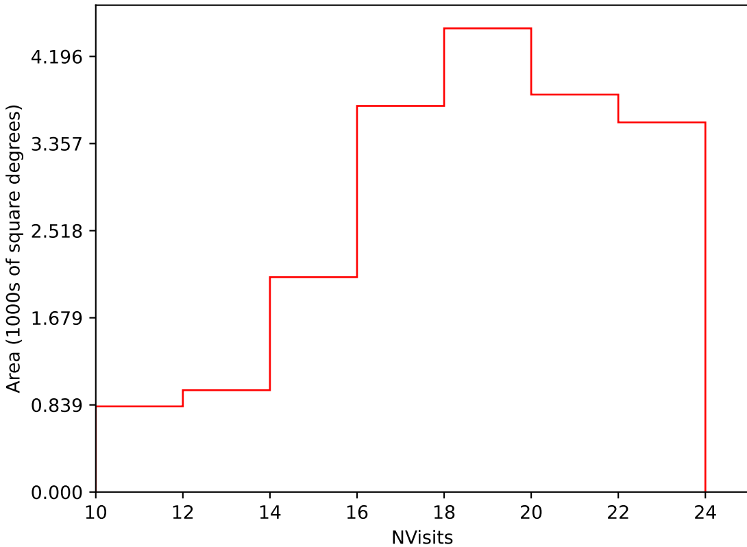
roll_pause_mjdp270_v3.4_10yrs Yr 1 i band: NVisits
