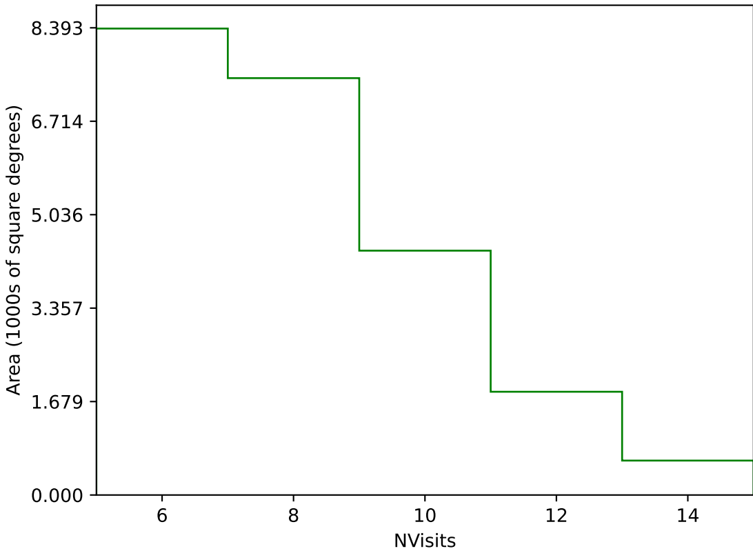
roll_pause_mjdp270_v3.4_10yrs Yr 1 g band: NVisits
