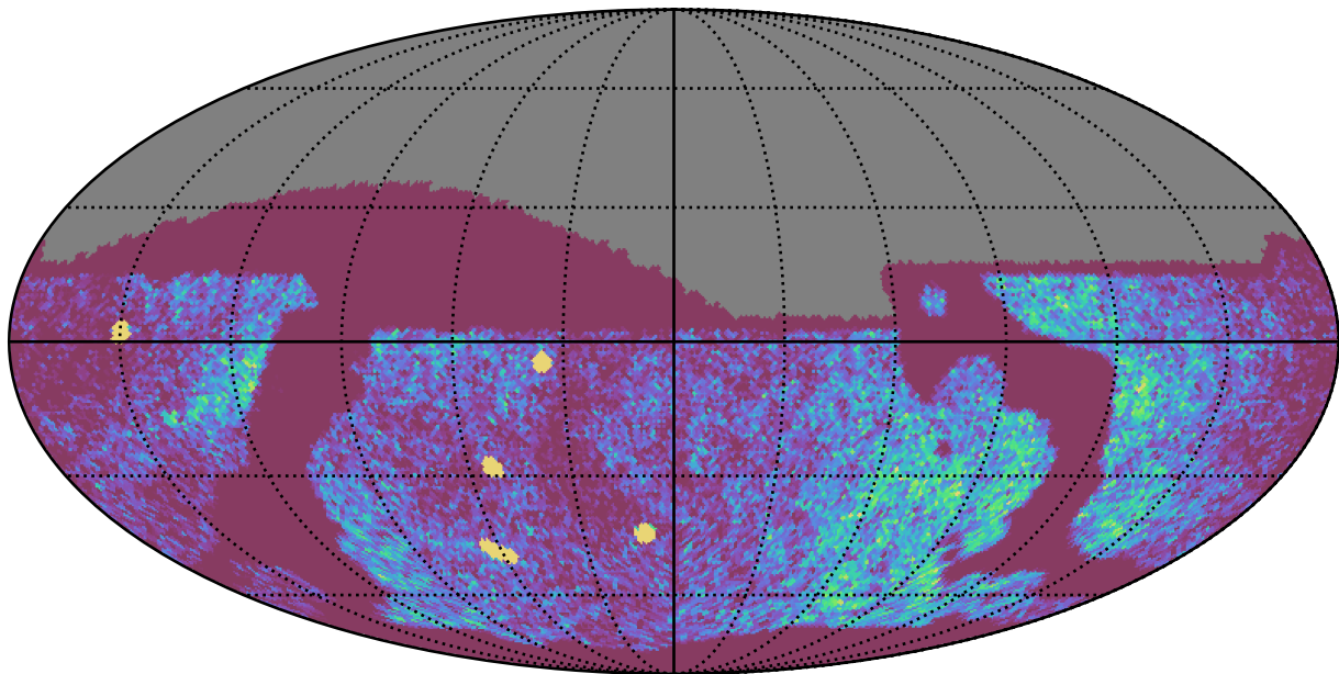
roll_pause_mjdp270_v3.4_10yrs Yr 1 all bands: NVisits
