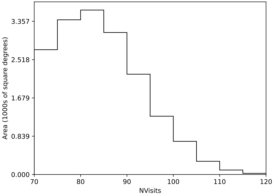
roll_pause_mjdp270_v3.4_10yrs Yr 1 all bands: NVisits
