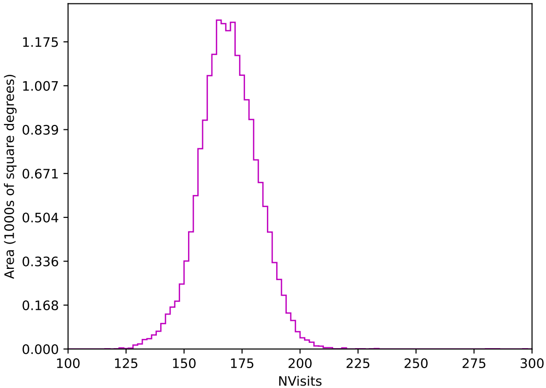
roll_pause_mjdp270_v3.4_10yrs WFD z band: NVisits
