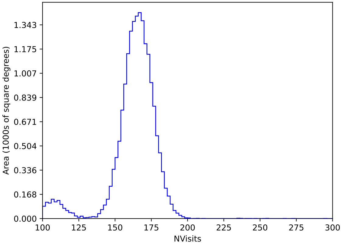
roll_pause_mjdp270_v3.4_10yrs WFD y band: NVisits
