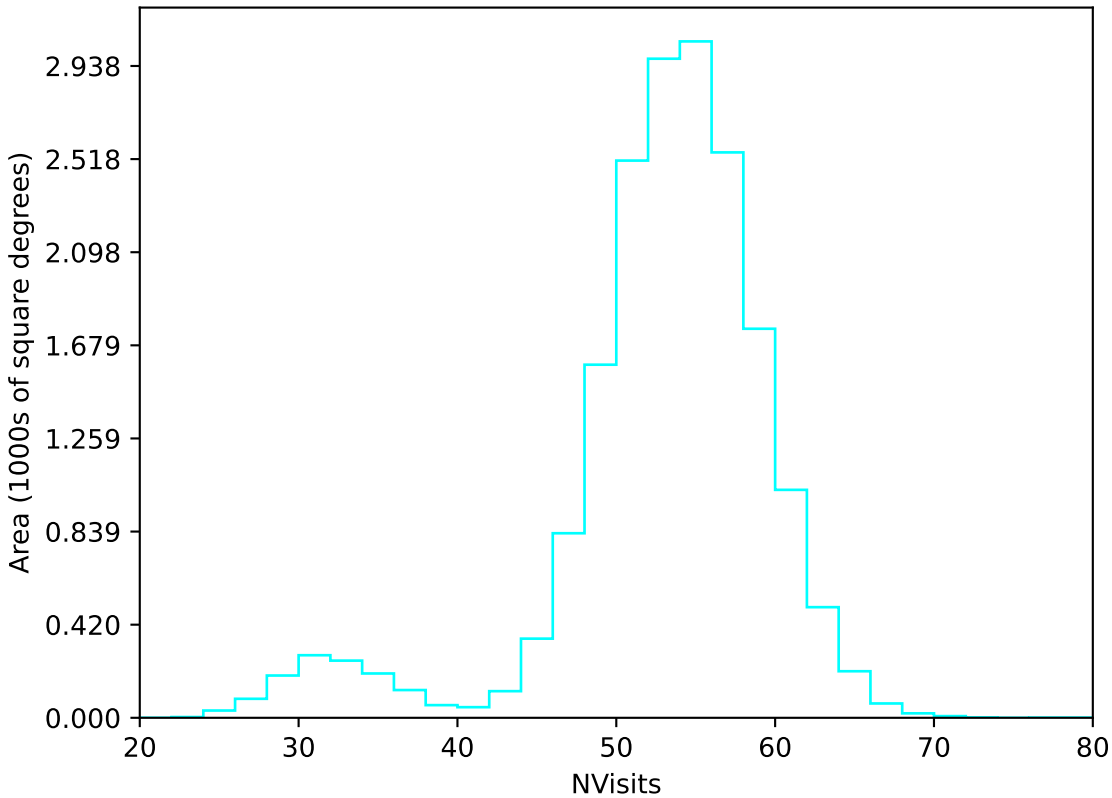
roll_pause_mjdp270_v3.4_10yrs WFD u band: NVisits
