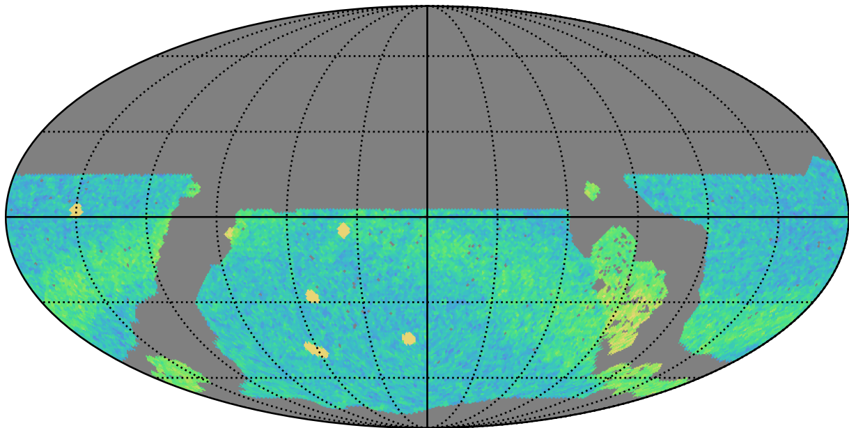
roll_pause_mjdp270_v3.4_10yrs WFD r band: NVisits
