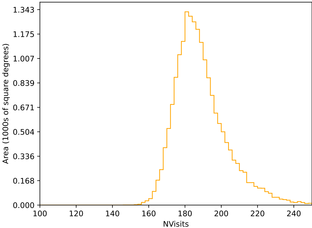
roll_pause_mjdp270_v3.4_10yrs WFD r band: NVisits
