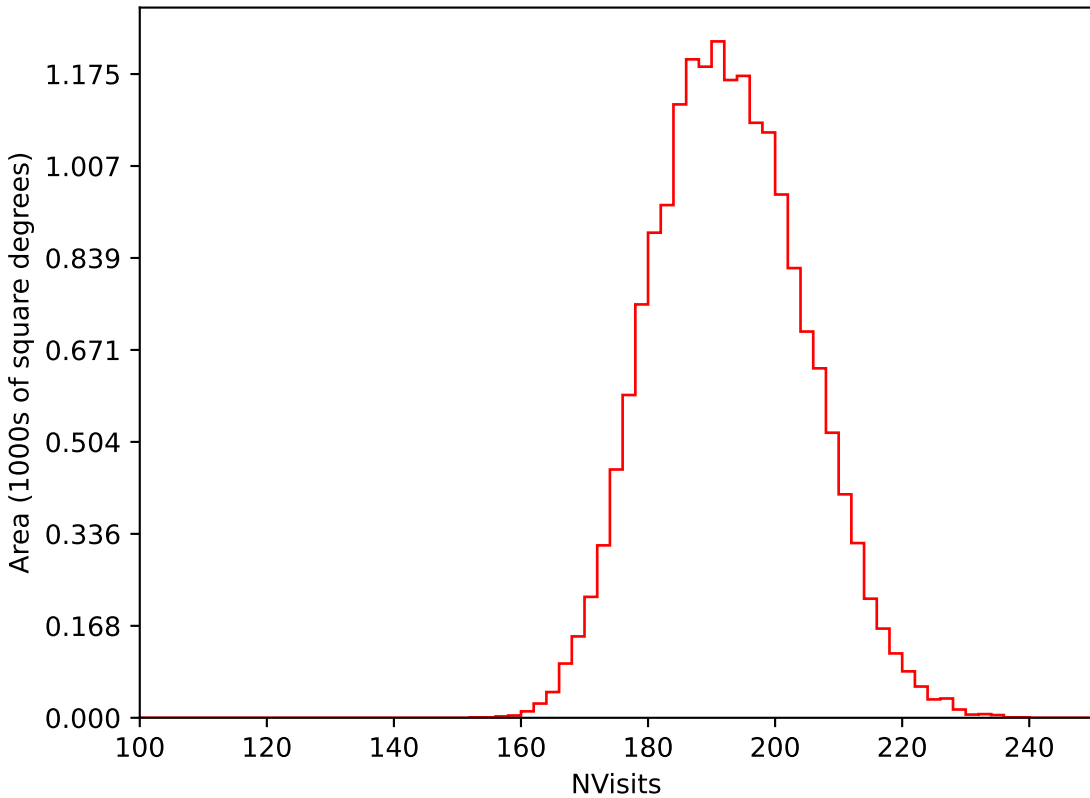
roll_pause_mjdp270_v3.4_10yrs WFD i band: NVisits
