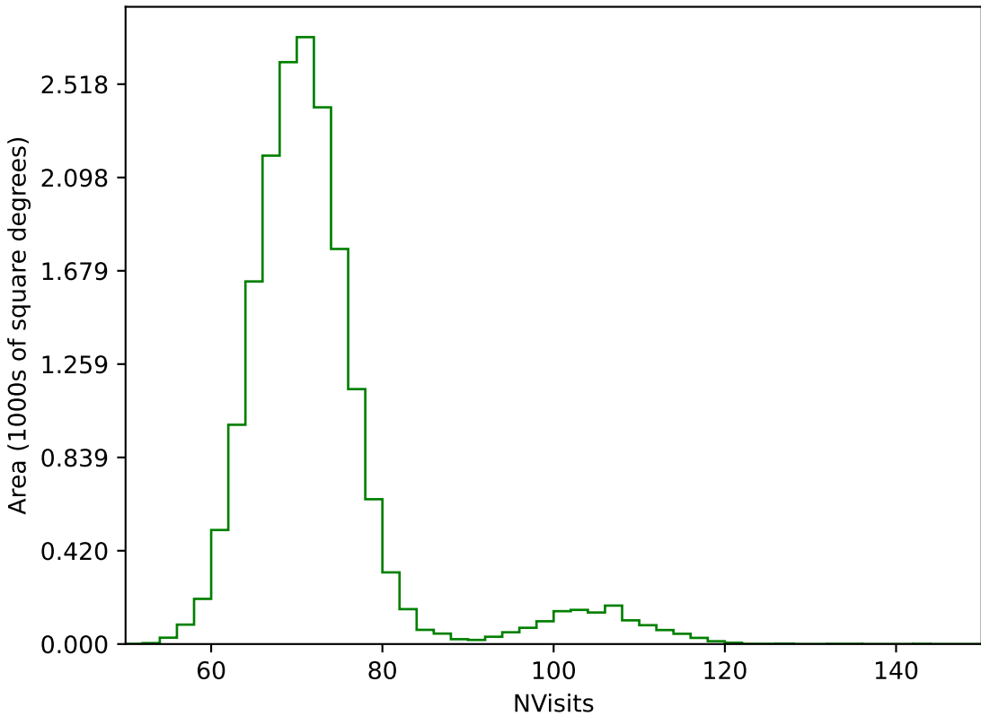
roll_pause_mjdp270_v3.4_10yrs WFD g band: NVisits
