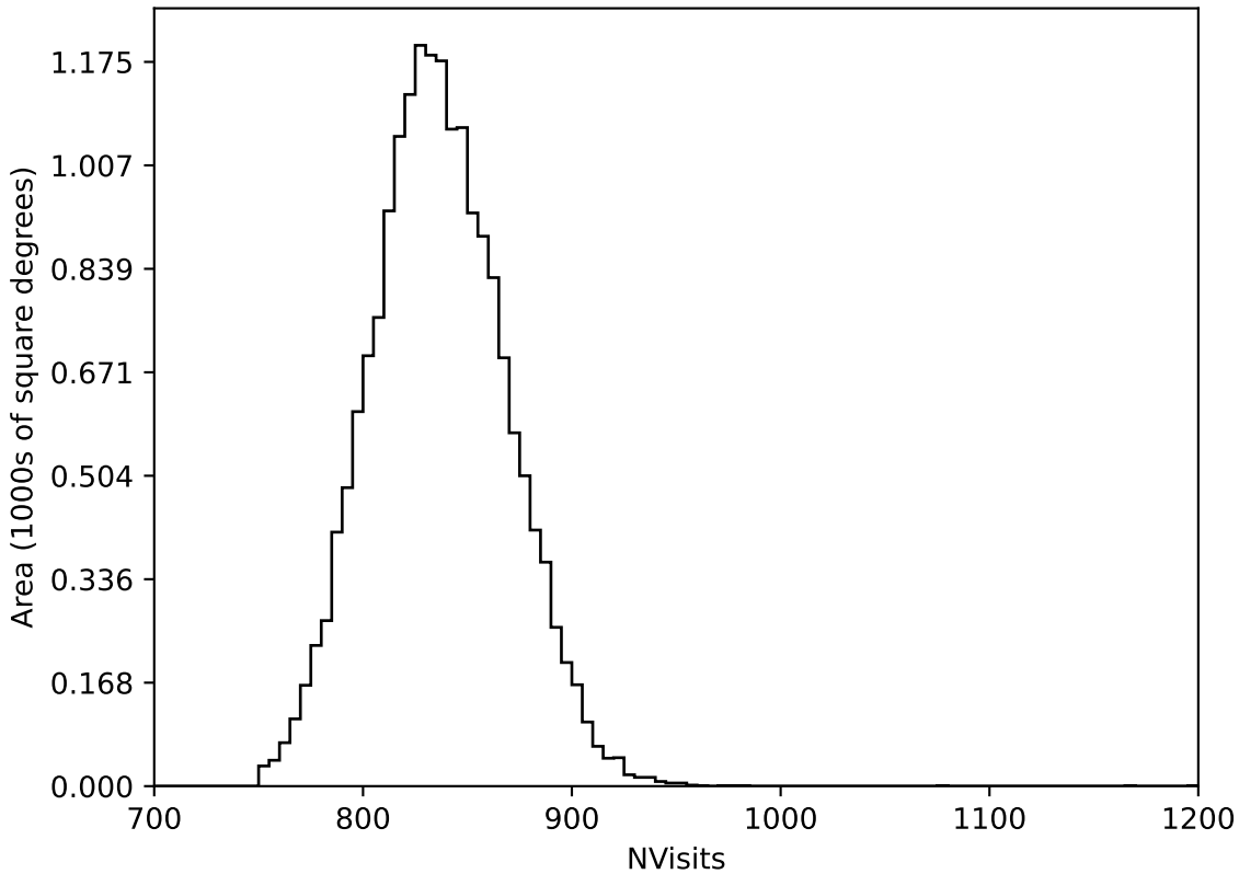
roll_pause_mjdp270_v3.4_10yrs WFD all bands: NVisits
