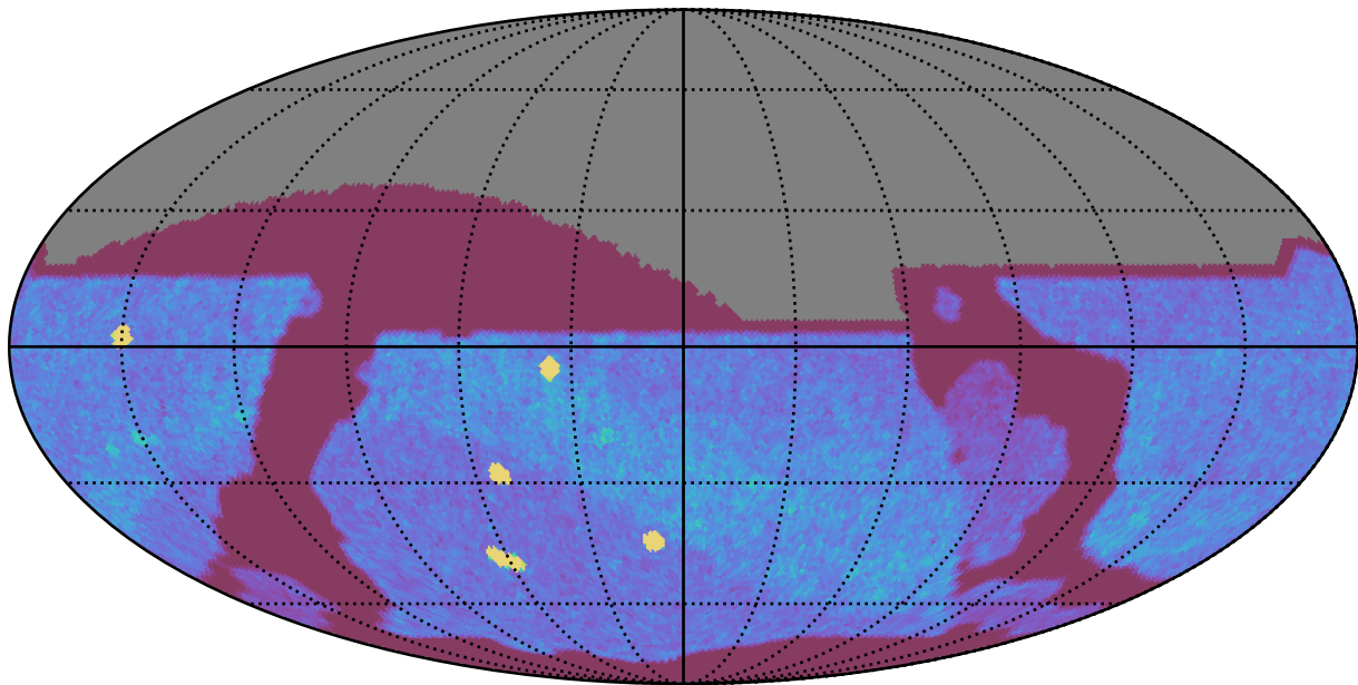
roll_pause_mjdp270_v3.4_10yrs All sky z band: NVisits
