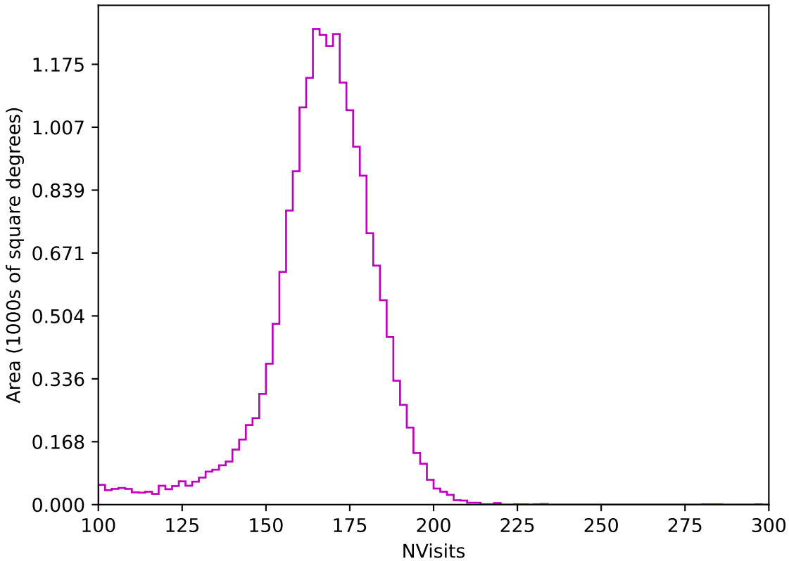
roll_pause_mjdp270_v3.4_10yrs All sky z band: NVisits
