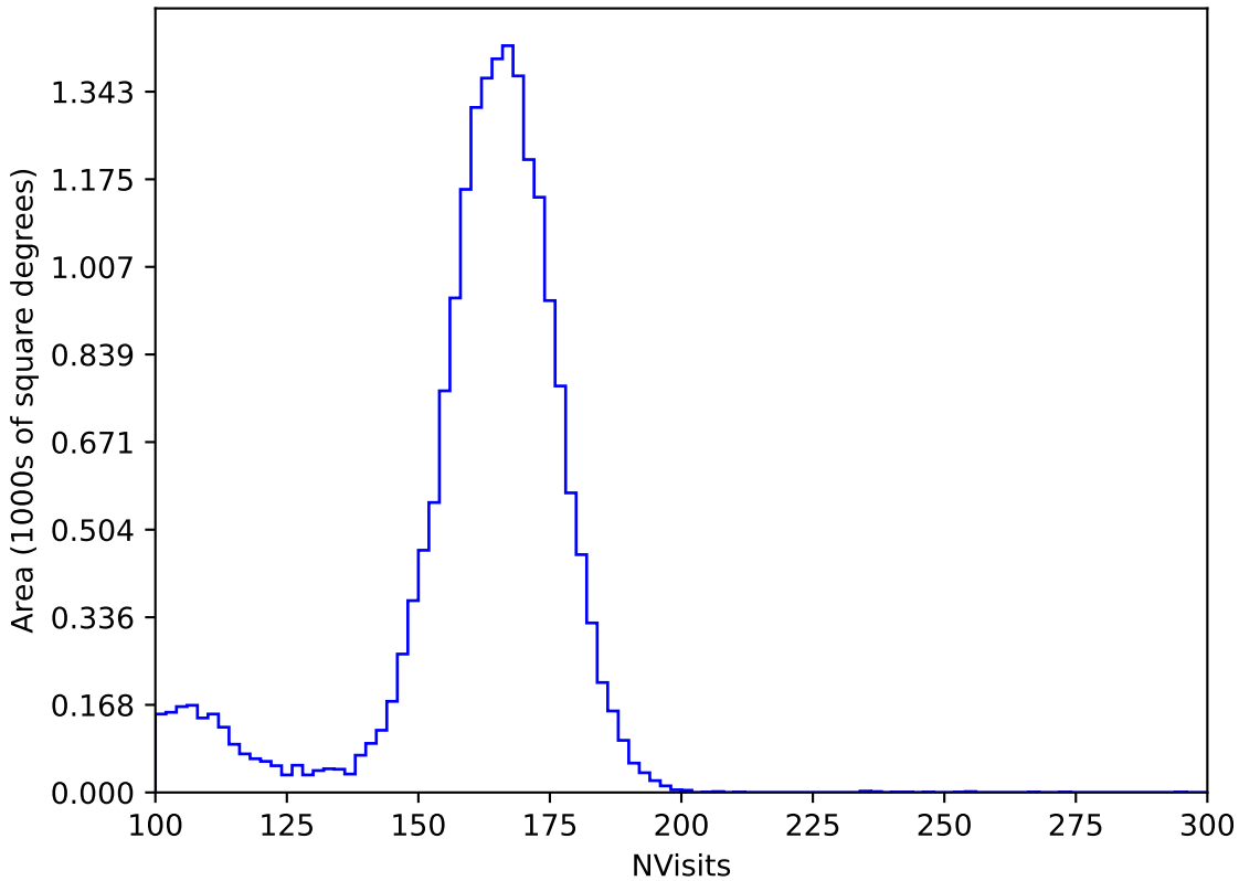
roll_pause_mjdp270_v3.4_10yrs All sky y band: NVisits
