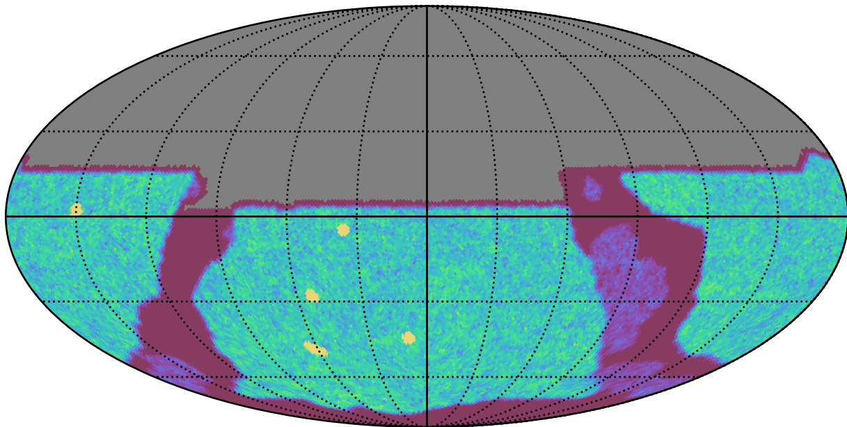
roll_pause_mjdp270_v3.4_10yrs All sky u band: NVisits
