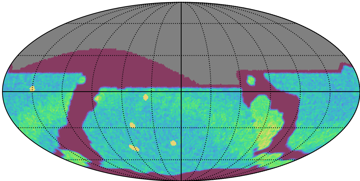
roll_pause_mjdp270_v3.4_10yrs All sky r band: NVisits
