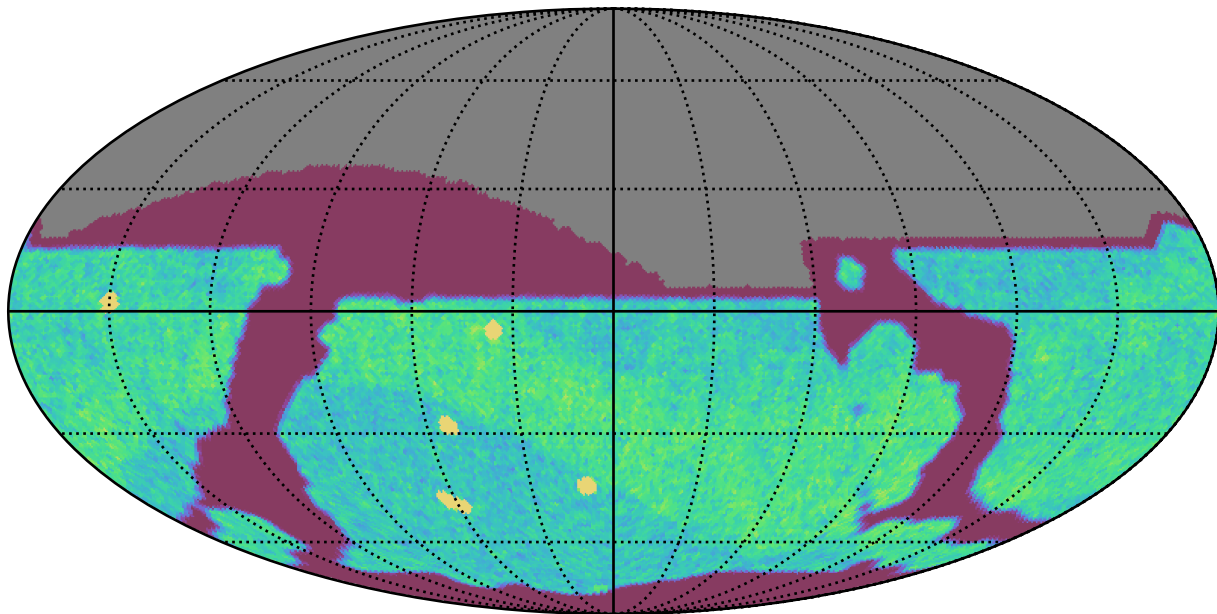
roll_pause_mjdp270_v3.4_10yrs All sky i band: NVisits
