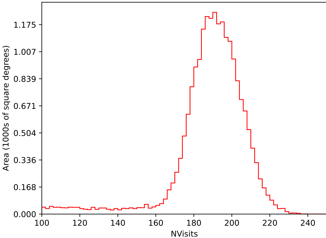
roll_pause_mjdp270_v3.4_10yrs All sky i band: NVisits
