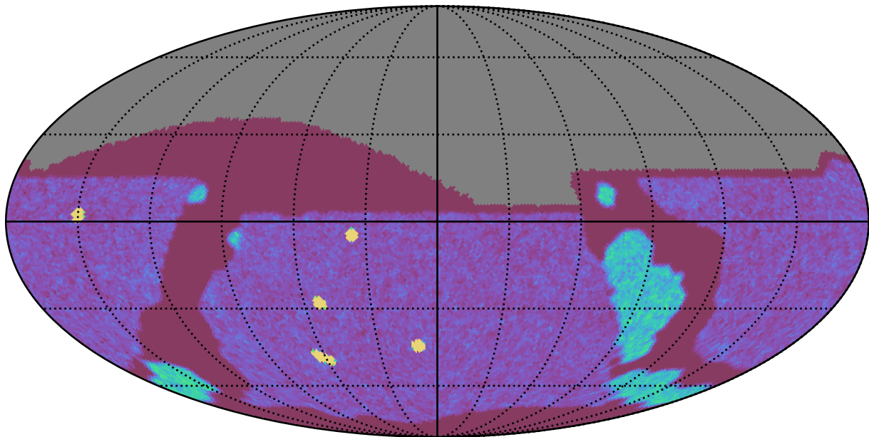
roll_pause_mjdp270_v3.4_10yrs All sky g band: NVisits
