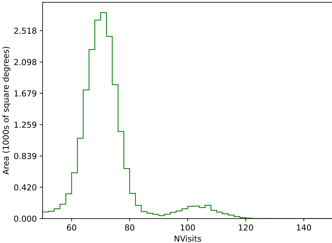
roll_pause_mjdp270_v3.4_10yrs All sky g band: NVisits
