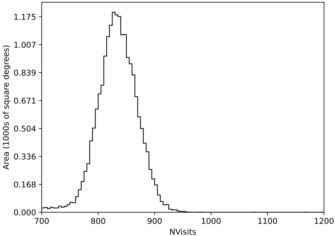
roll_pause_mjdp270_v3.4_10yrs All sky all bands: NVisits
