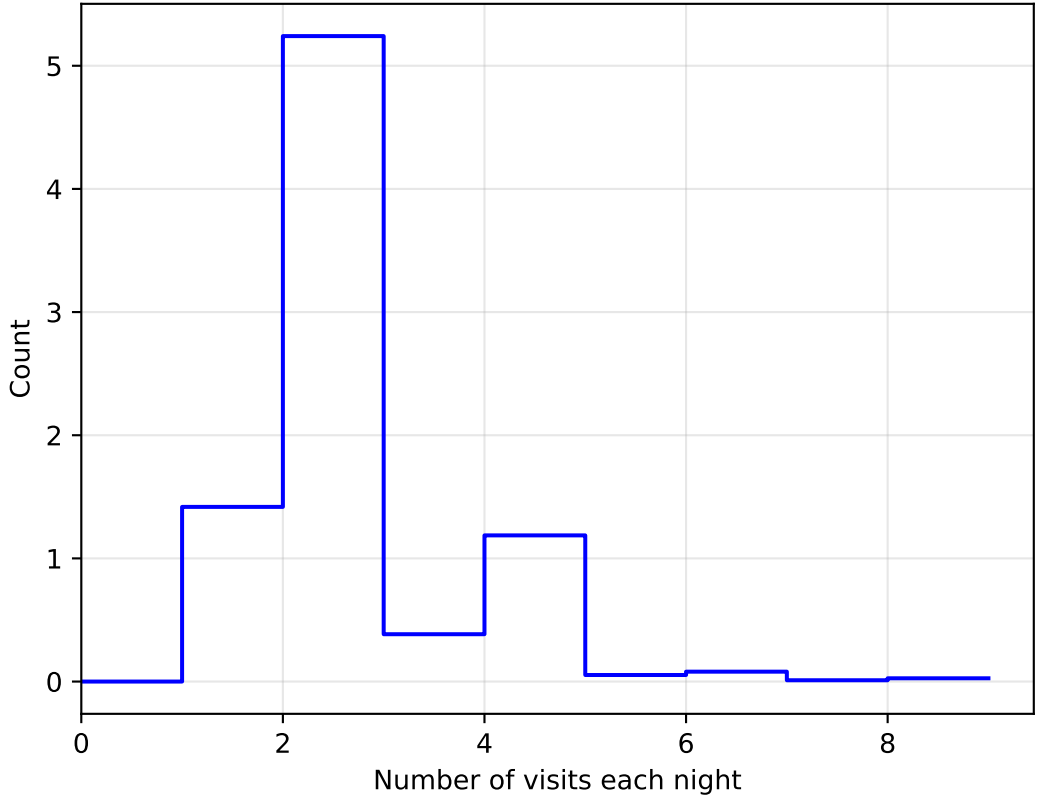
roll_pause_mjdp270_v3.4_10yrs WFD: NVisitsPerNight
