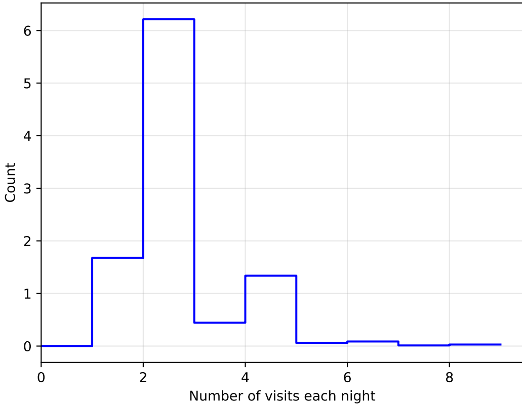
roll_pause_mjdp270_v3.4_10yrs All sky: NVisitsPerNight
