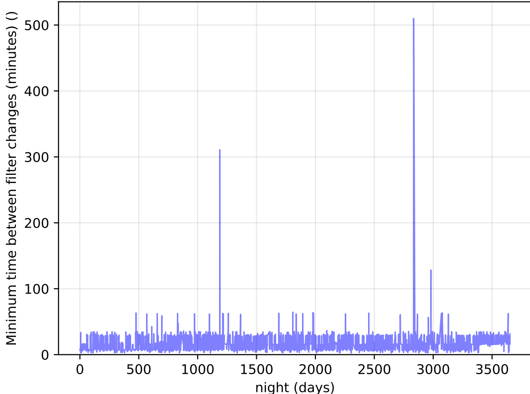
roll_pause_mjdp270_v3.4_10yrs Per Night: Minimum time between filter changes (minutes)
