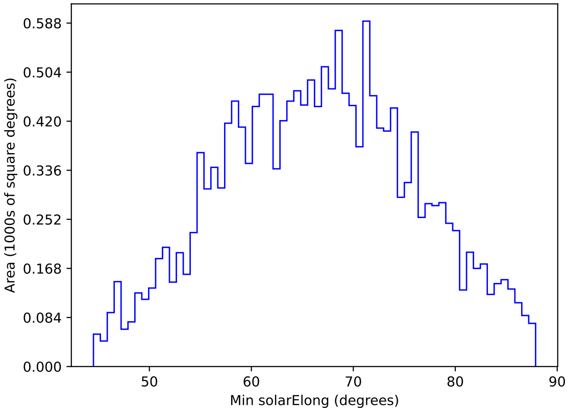
roll_pause_mjdp270_v3.4_10yrs WFD y band: Min solarElong
