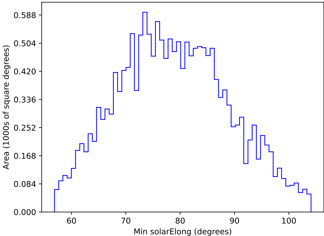
roll_pause_mjdp270_v3.4_10yrs WFD u band: Min solarElong
