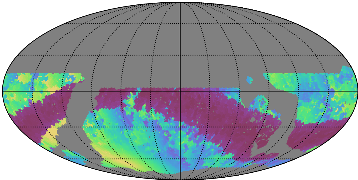
roll_pause_mjdp270_v3.4_10yrs WFD r band: Min solarElong
