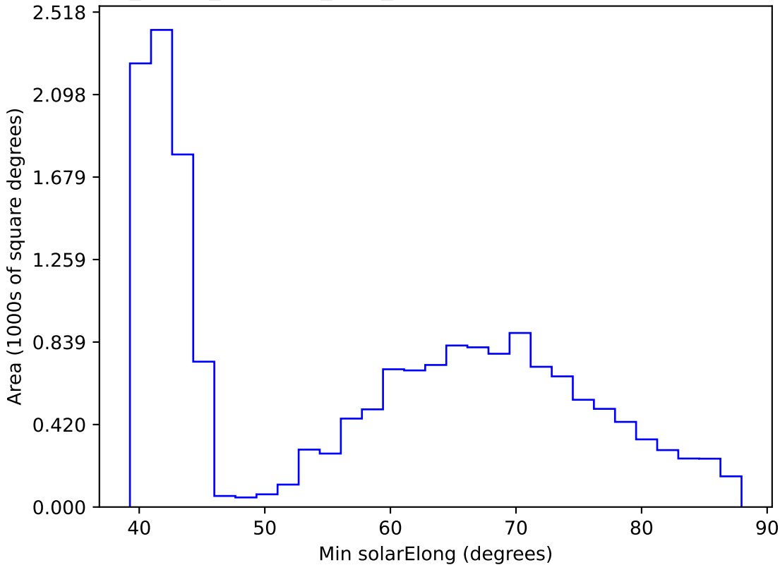
roll_pause_mjdp270_v3.4_10yrs WFD r band: Min solarElong
