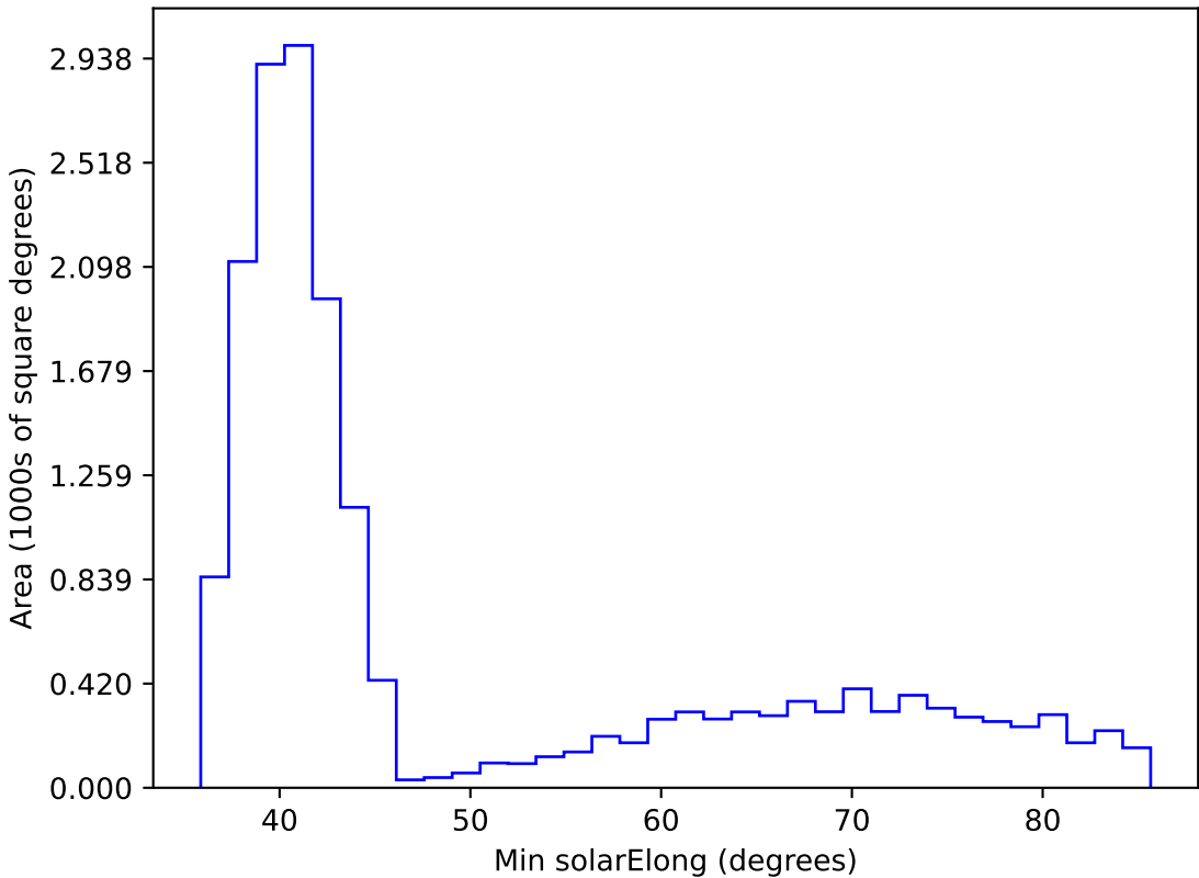
roll_pause_mjdp270_v3.4_10yrs WFD i band: Min solarElong
