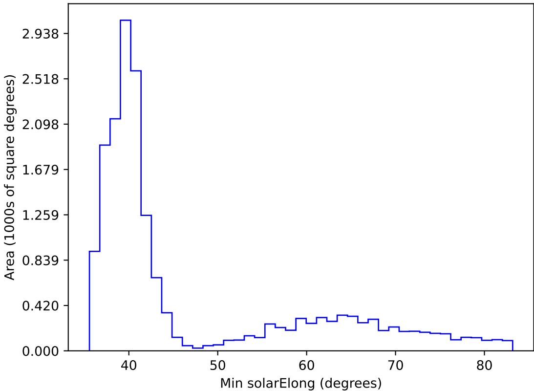
roll_pause_mjdp270_v3.4_10yrs WFD all bands: Min solarElong
