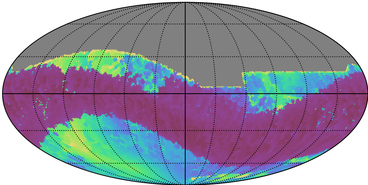
roll_pause_mjdp270_v3.4_10yrs All sky z band: Min solarElong
