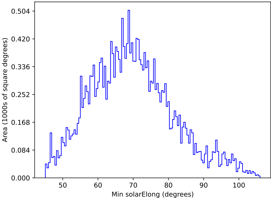
roll_pause_mjdp270_v3.4_10yrs All sky y band: Min solarElong
