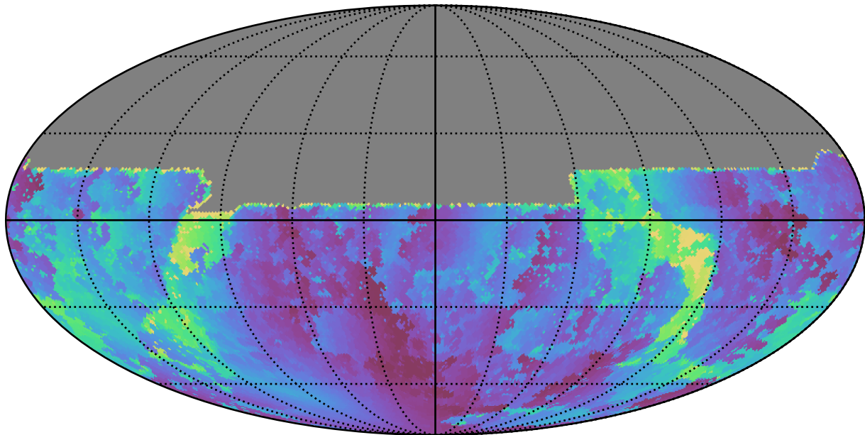
roll_pause_mjdp270_v3.4_10yrs All sky u band: Min solarElong
