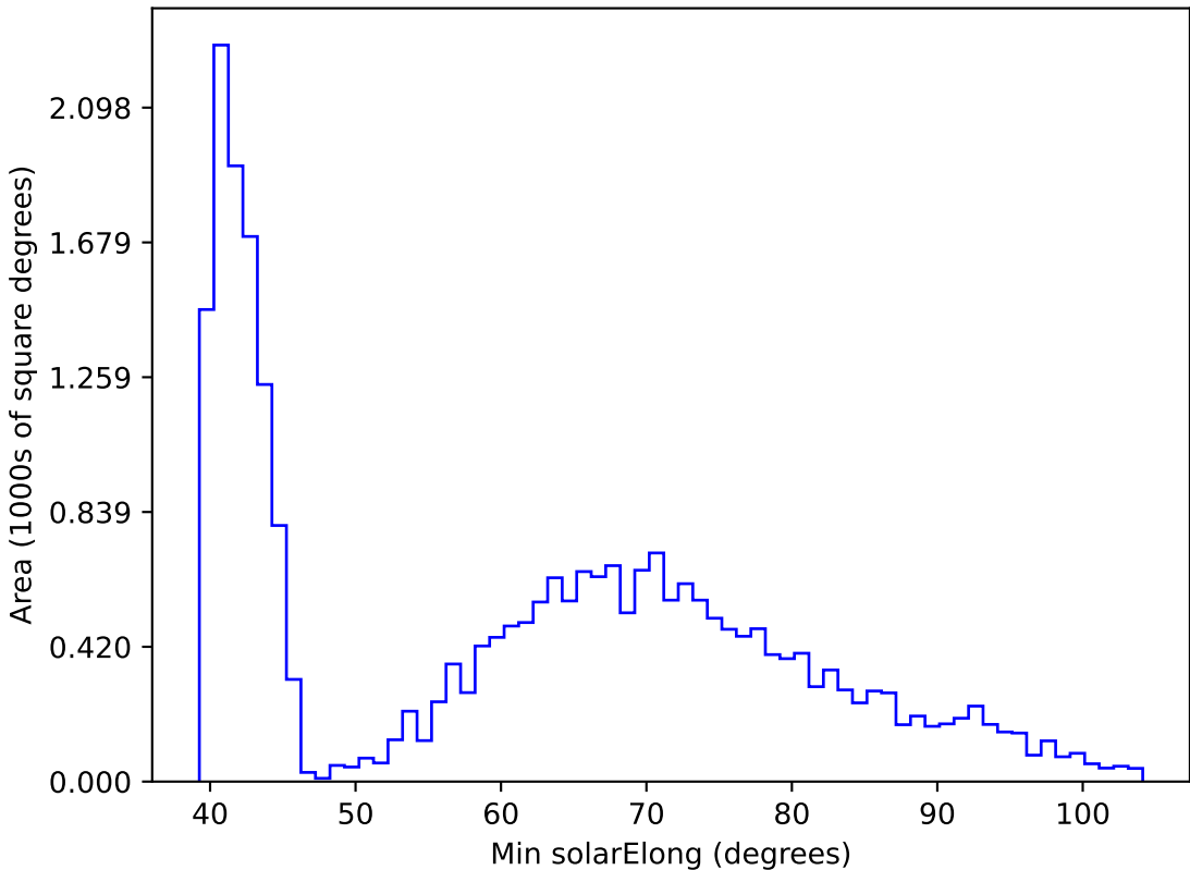
roll_pause_mjdp270_v3.4_10yrs All sky r band: Min solarElong
