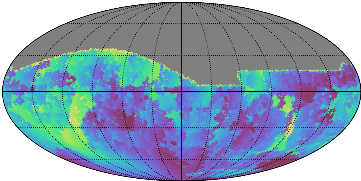
roll_pause_mjdp270_v3.4_10yrs All sky g band: Min solarElong
