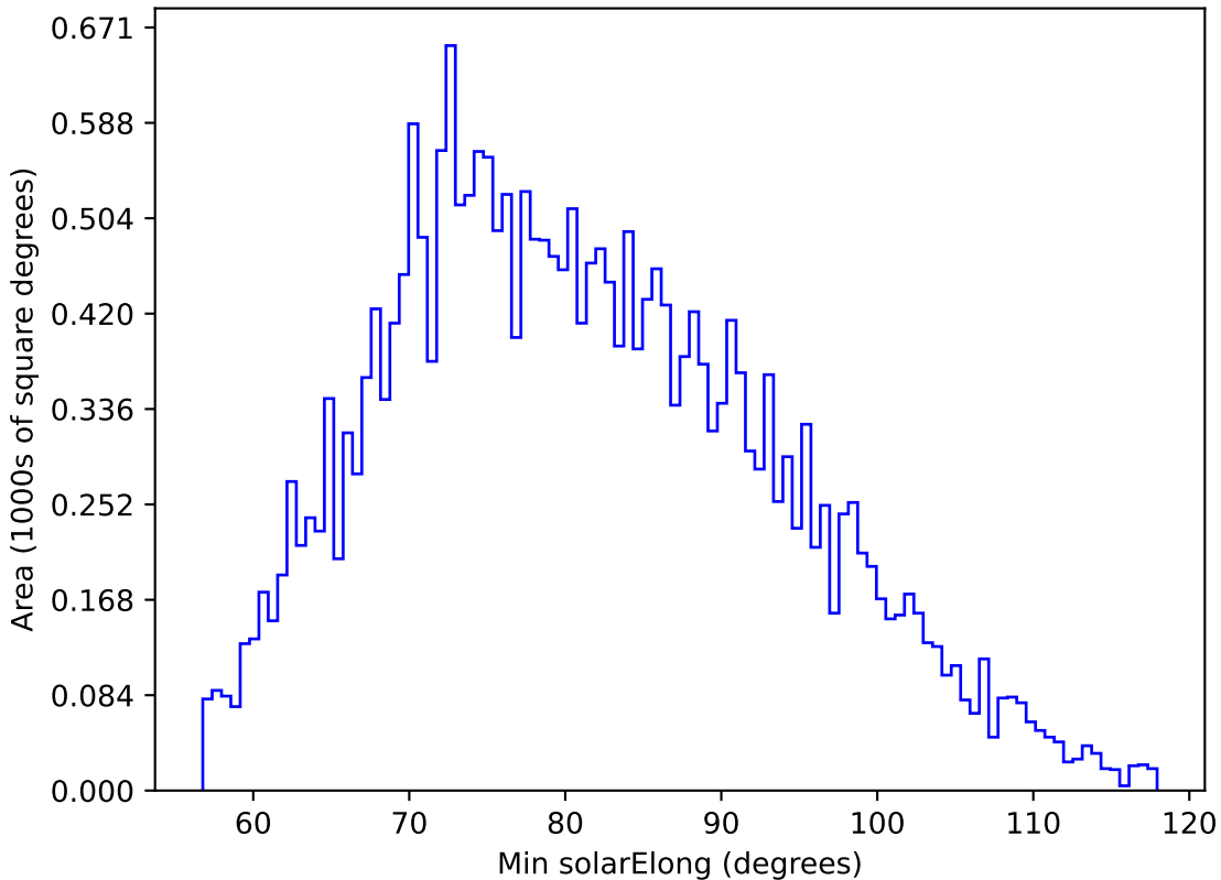
roll_pause_mjdp270_v3.4_10yrs All sky g band: Min solarElong
