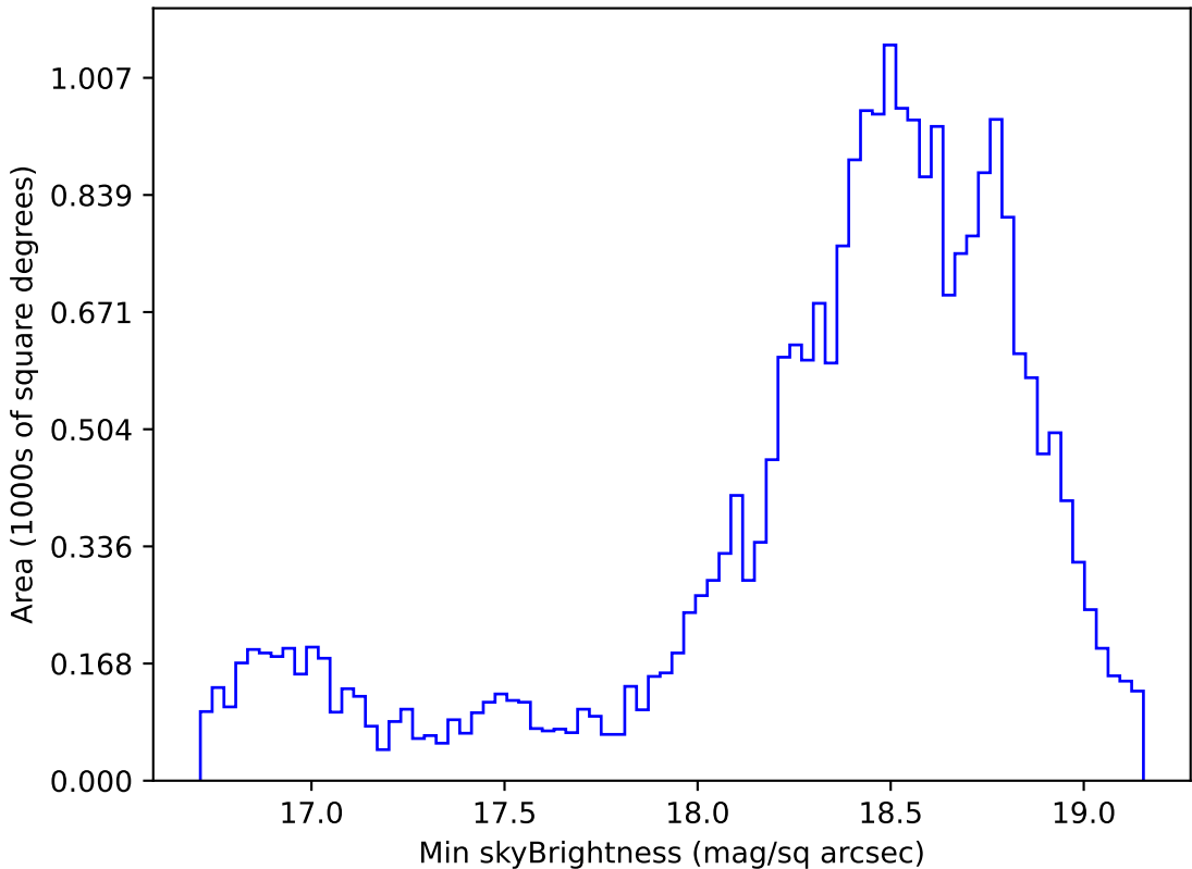
roll_pause_mjdp270_v3.4_10yrs Yr 1 z band: Min skyBrightness
