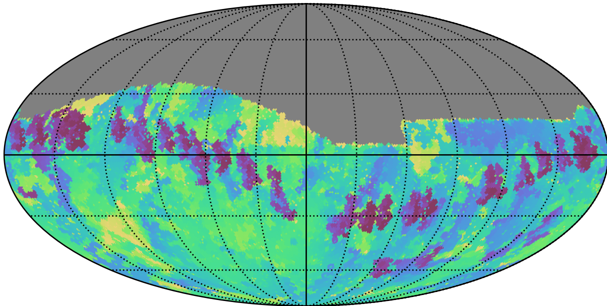
roll_pause_mjdp270_v3.4_10yrs Yr 1 i band: Min skyBrightness
