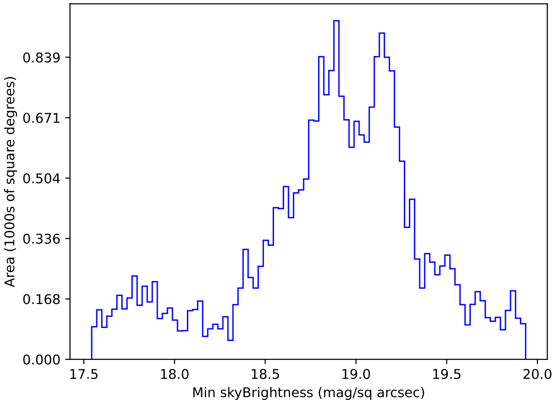
roll_pause_mjdp270_v3.4_10yrs Yr 1 i band: Min skyBrightness
