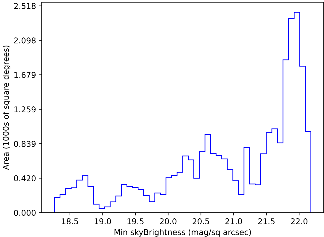
roll_pause_mjdp270_v3.4_10yrs Yr 1 g band: Min skyBrightness
