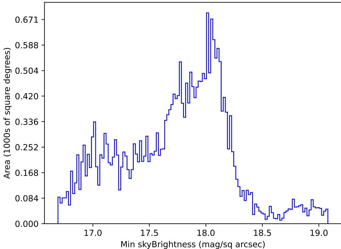
roll_pause_mjdp270_v3.4_10yrs Yr 1 all bands: Min skyBrightness
