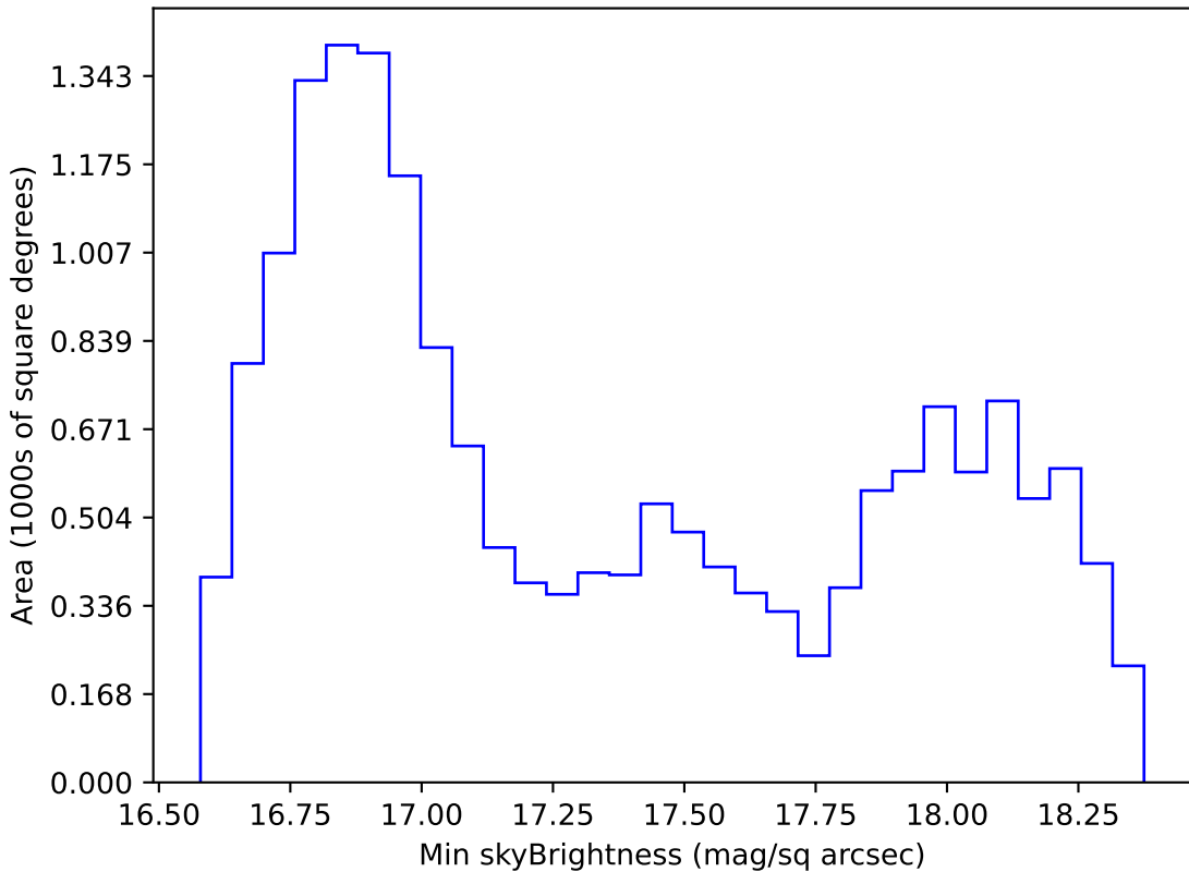
roll_pause_mjdp270_v3.4_10yrs WFD z band: Min skyBrightness
