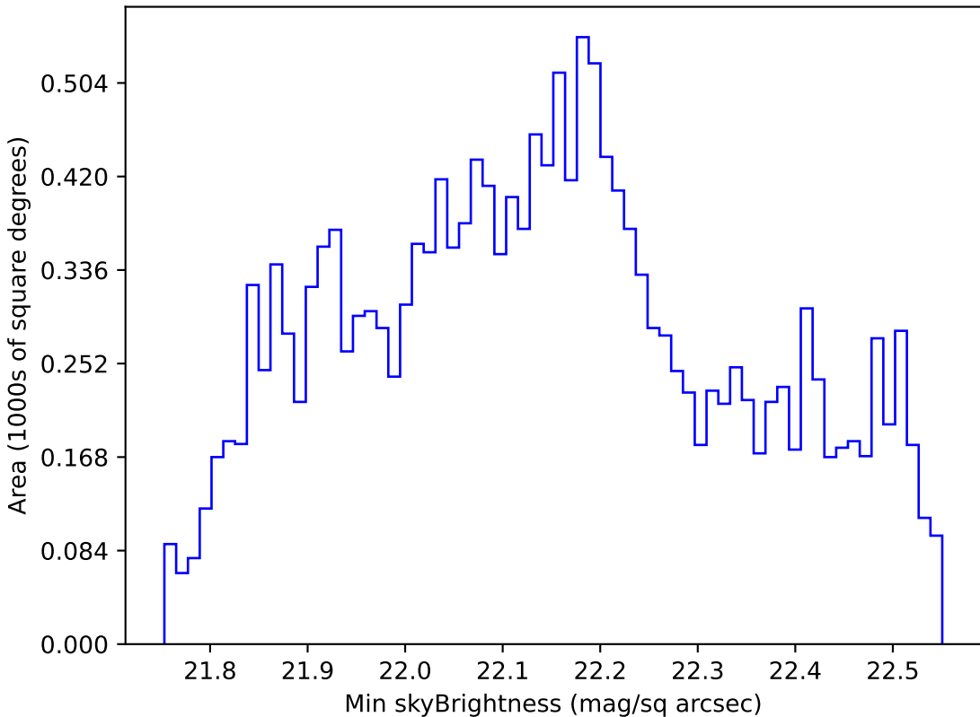
roll_pause_mjdp270_v3.4_10yrs WFD u band: Min skyBrightness
