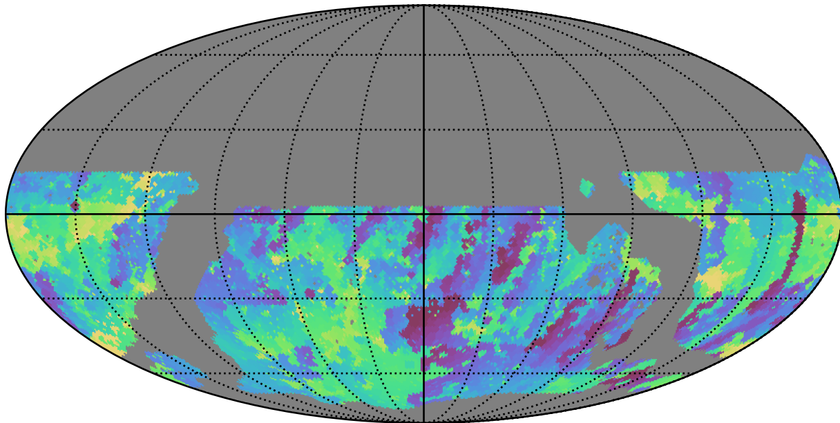
roll_pause_mjdp270_v3.4_10yrs WFD r band: Min skyBrightness
