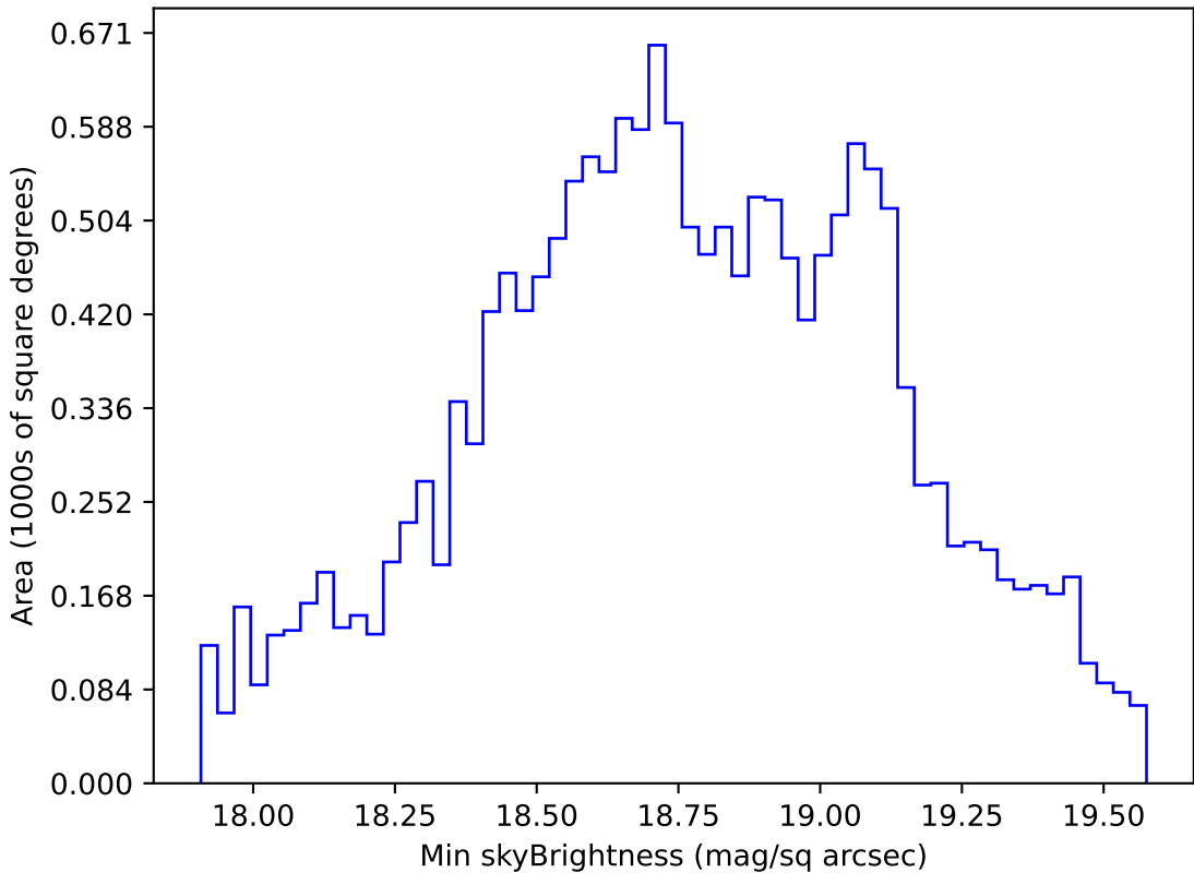
roll_pause_mjdp270_v3.4_10yrs WFD r band: Min skyBrightness
