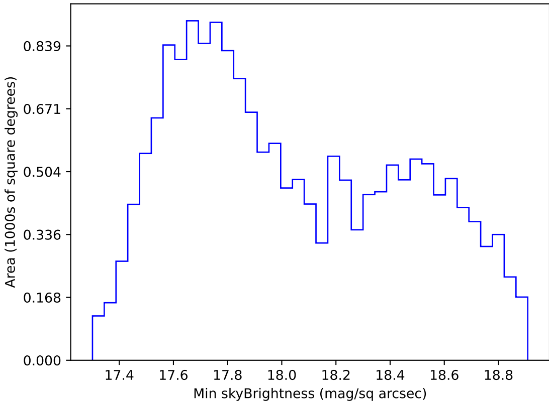
roll_pause_mjdp270_v3.4_10yrs WFD i band: Min skyBrightness
