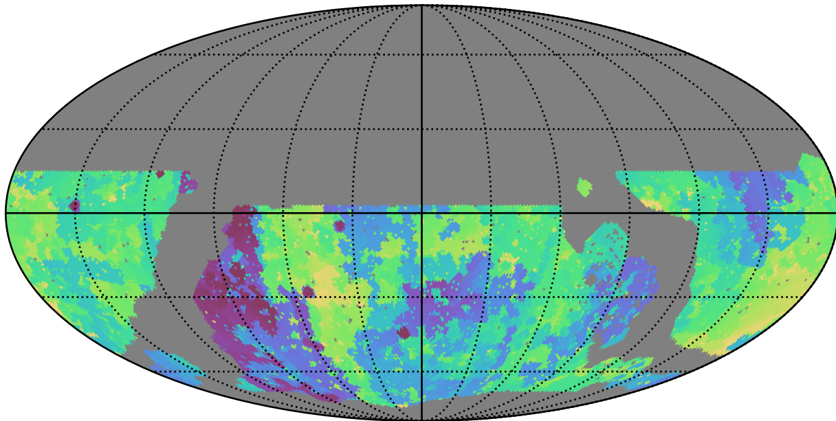
roll_pause_mjdp270_v3.4_10yrs WFD g band: Min skyBrightness
